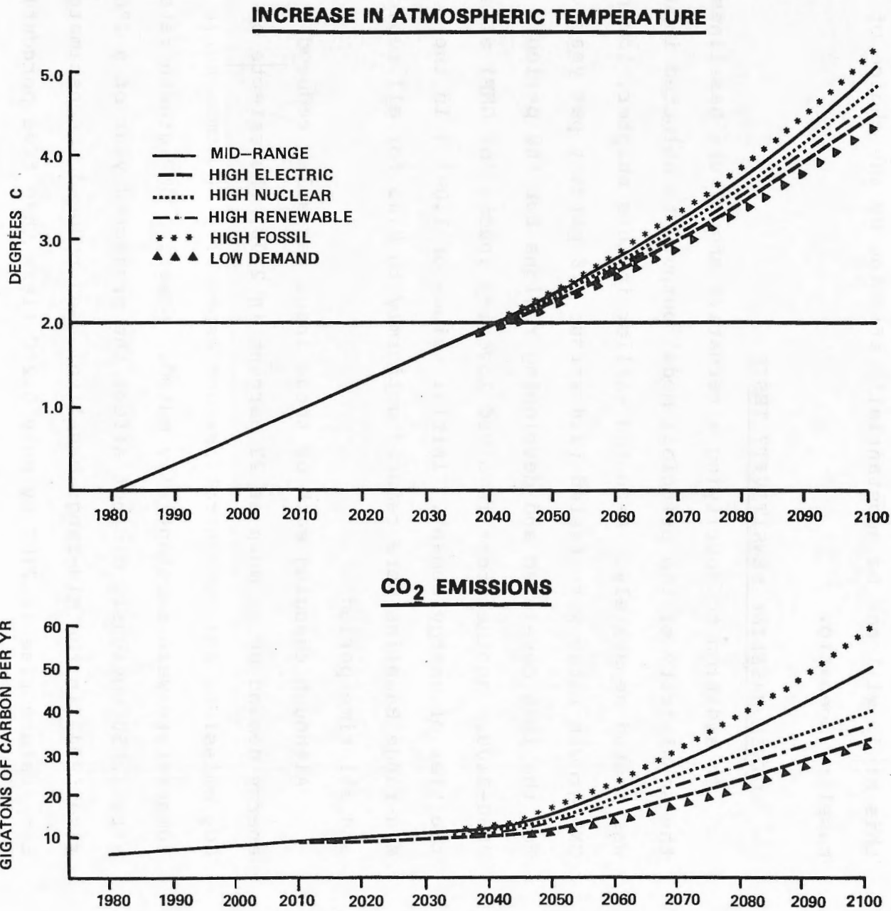
FIGURE 4-10 CO 2 MODELING RESULTS FOR ALTERNATIVE BASELINE SCENARIOS
